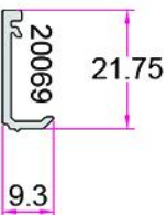
زهوار TS94-TS77 Glazing Bead 0.135Kg/m
